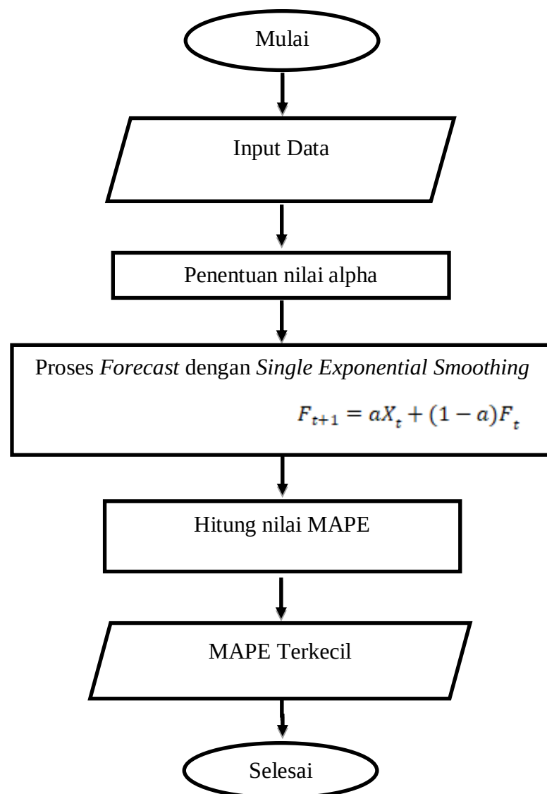
Gambar 3.1 Flowchart Single Ekspponential Smoothing
